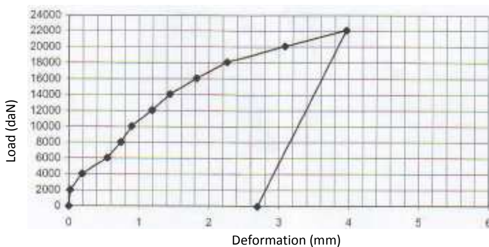
Graphic : load vs deformation
